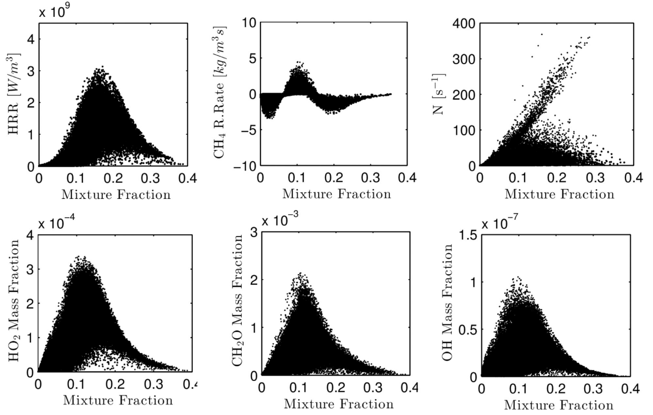
Fig. 6. Scatter plots of heat release rate (HRR), \text{CH}_4 reaction rate, scalar dissipation rate ( N ) and mass fractions of \text{CH}_2\text{O} , \text{OH} and \text{HO}_2 at t = 0.650 ms. Data shown correspond to case A.
