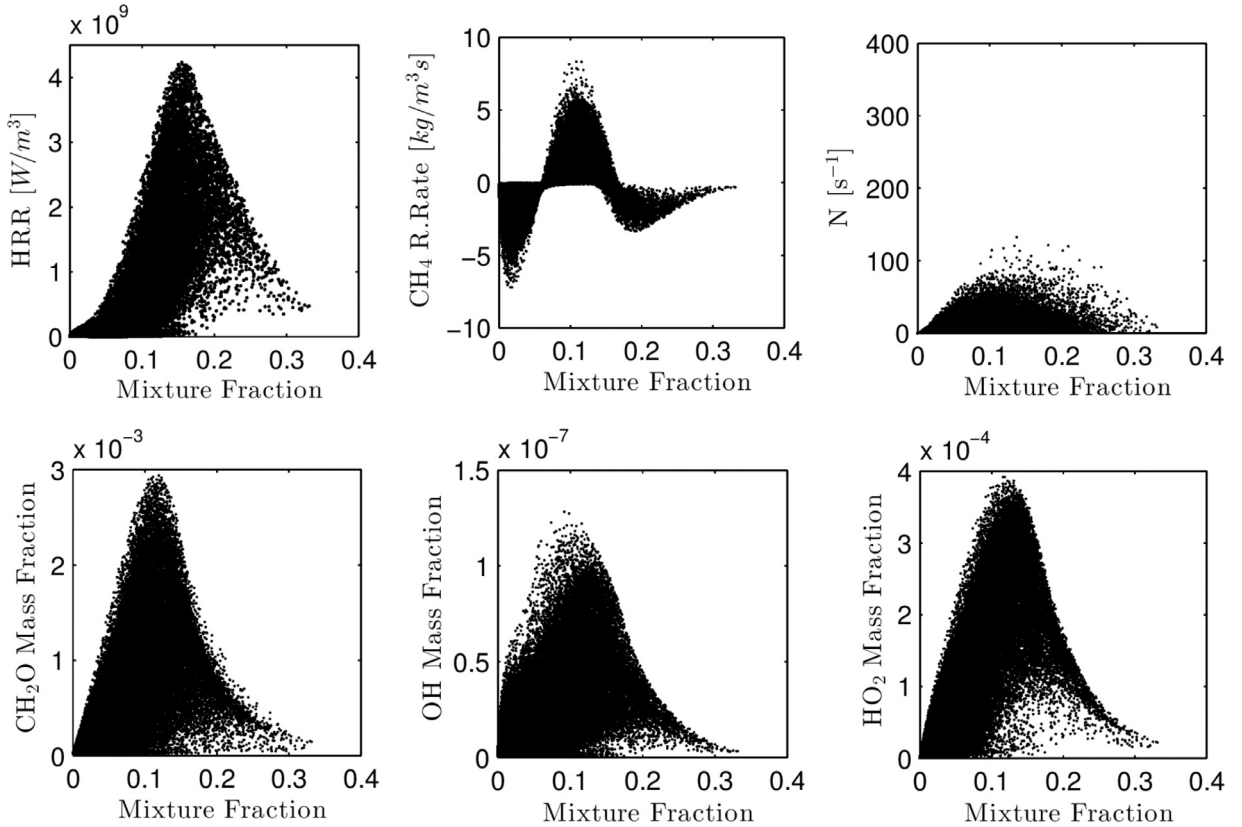
Fig. 7. Scatter plots of heat release rate (HRR), \text{CH}_4 reaction rate, scalar dissipation rate ( N ) and mass fractions of \text{CH}_2\text{O} , \text{OH} and \text{HO}_2 at t = 0.650 ms. Data shown correspond to case B.
