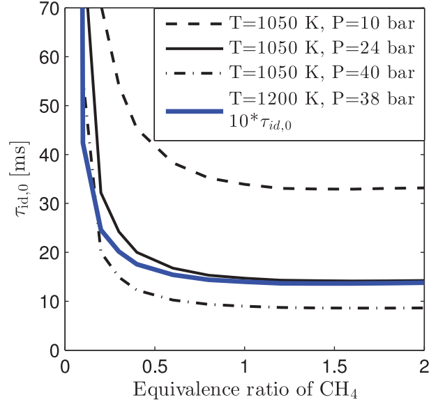
Fig. 3. Ignition delay time of \xi = 0 ( \tau_{id,0} ) against \phi_{CH_4} under different pressures. The value of the \tau_{id,0} is also computed for adiabatic compression conditions from P_0 = 24 bar ( T_0 = 1050 K) to P_{fin} = 38 bar ( T_{fin} = 1200 K).
