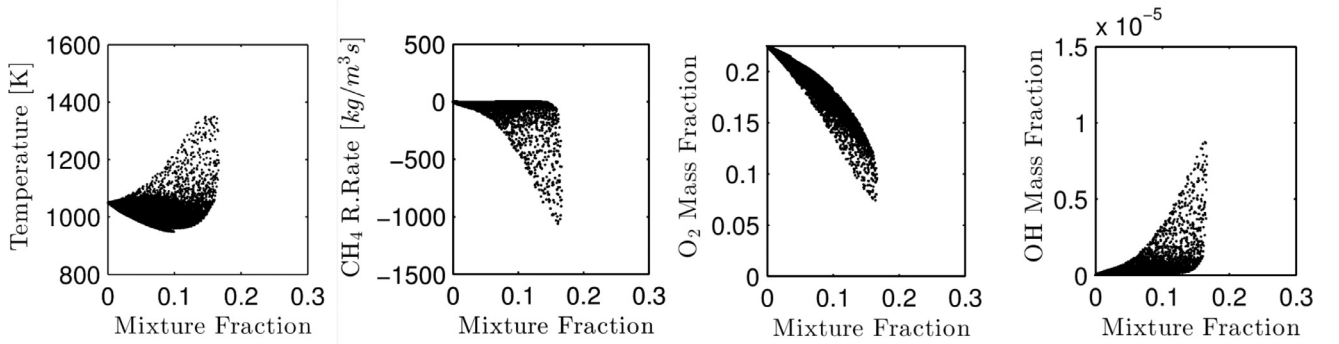
Fig. 10. Scatter plots of temperature, CH 4 reaction rate, and mass fractions of O 2 and OH taken at the ignition time of case B, \tau_{id}^{DNS,B} = 1.148 ms.
