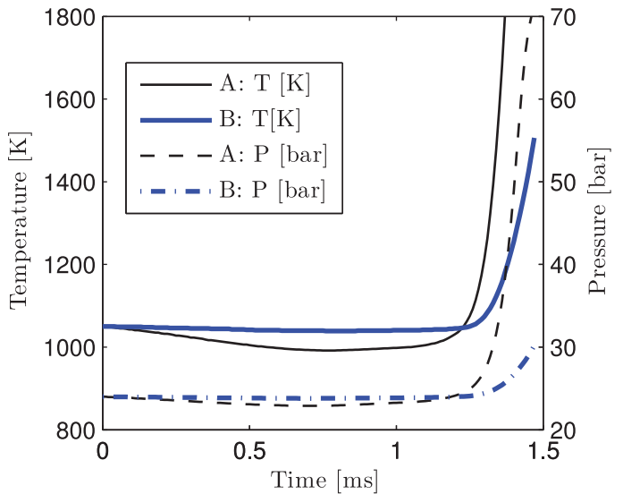
Fig. 5. Temporal evolution of volume averaged temperature and pressure for the DNS cases A and B.
