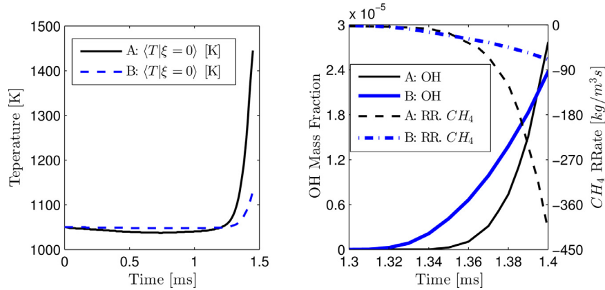
Fig. 14. Temporal evolution of (left) \langle T|\xi=0 \rangle and (right) methane reaction rate \langle \text{RR.CH}_4|\xi=0 \rangle and OH mass fraction \langle Y_{\text{OH}}|\xi=0 \rangle , for both cases, conditional on \xi=0 .
