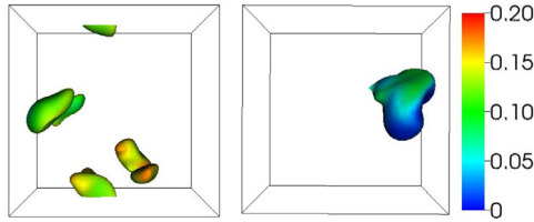
Fig. 11. Iso-surface of T = 1250 K coloured by mixture fraction, soon after the first appearance of ignition. Case A (left): t = 1.16 ms. Case B (right): t = 1.30 ms.
