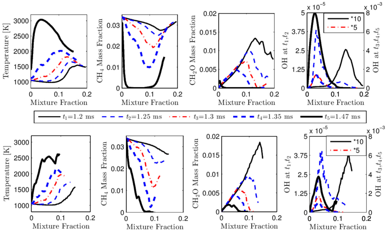
Fig. 13. Conditional averages of temperature, and \text{CH}_4 , \text{CH}_2\text{O} , OH mass fractions at the indicated time instants for case A (upper) and B (lower).
