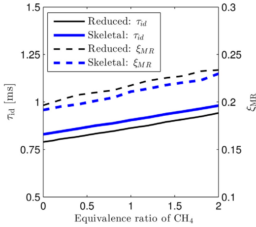
Fig. A.20. Reference ignition delay times ( \tau_{id} ) and most reactive mixture fractions ( \xi_{MR} ) predicted from the reduced and skeletal scheme. The pressure and temperature of the oxidiser and n-heptane streams are the same as the DNS conditions ( P = 24 bar, T_{ox} = 1050 K, T_f = 450 K).
