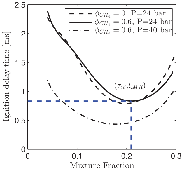
Fig. 2. Ignition delay time of homogeneous n-heptane/oxidizer mixtures, where the oxidizer ( \xi = 0 ) is a methane–air mixture at the indicated equivalence ratio ( \phi_{CH_4} ) and T_{ox} = 1050 K. Each mixture initial condition is determined from inert mixing of the oxidiser and the n-heptane fuel stream ( \xi = 1 , T_F = 450 K). For each set of conditions the shortest ignition delay time, namely \tau_{id} , is observed for a mixture fraction denoted as \xi_{MR} .
