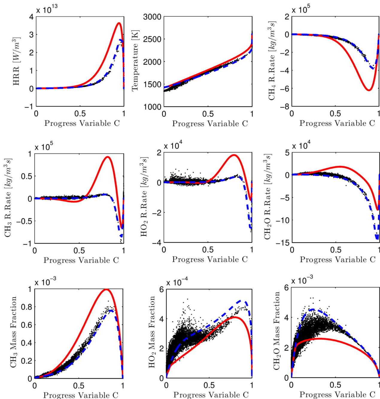
Fig. 17. Scatter plots of heat release rate (HRR), temperature, reaction rates of \text{CH}_4 , \text{CH}_3 , \text{HO}_2 , and \text{CH}_2\text{O} and mass fractions of \text{CH}_3 , \text{HO}_2 , and \text{CH}_2\text{O} at \xi = 0 , plotted against the progress variable C and compared with 1-D laminar premixed flame calculations (red continuous line) and homogeneous reactor calculations (blue dashed line). The DNS data (black points) are taken from case A at t = 1.47 ms. (For interpretation of the references to colour in this figure legend, the reader is referred to the web version of this article.)
