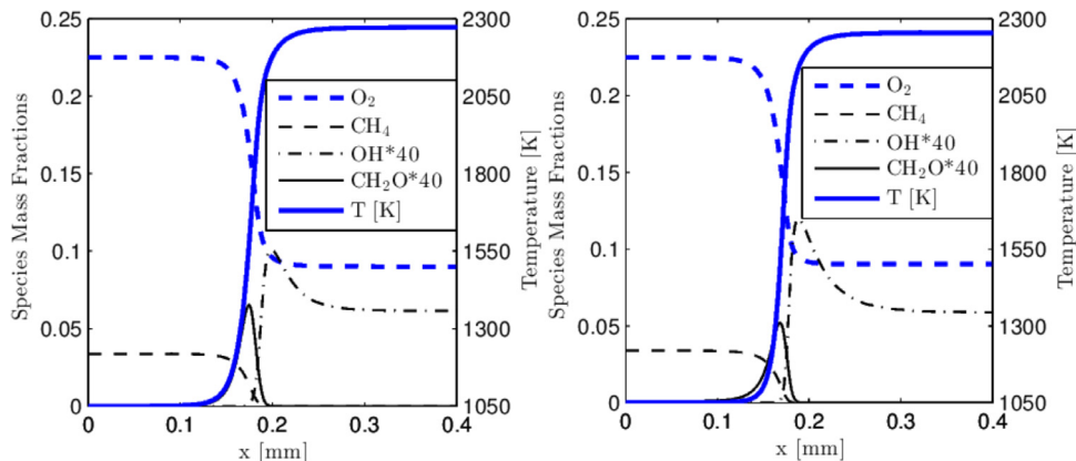
Fig. A.22. Species profiles computed using the GRI-3.0 mechanism [46] (left) and the Liu et al. (2004) [20] skeletal scheme (right) at the nominal conditions; P = 24 bar, T = 1050 K, \phi_{CH_4} = 0.6 .
