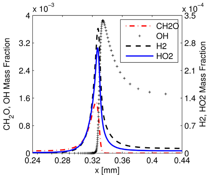
Fig. B.23. Species profiles of a laminar premixed methane/air flame at P = 27 bar, T = 1,080 K, \phi_{\text{CH}_4} = 0.6 using the Liu et al. (2004) chemical mechanism [20].
