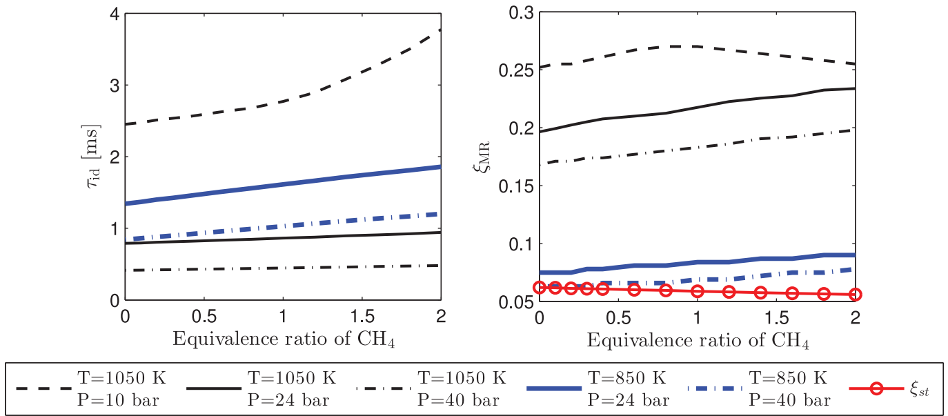
Fig. 4. Left: reference ignition delay time ( \tau_{id} ) of homogeneous n-heptane/oxidiser mixtures for a range of \phi_{\text{CH}_4} in the oxidiser stream. The value of the \tau_{id} is computed for different pressures and oxidiser ( \xi = 0 ) temperatures while the n-heptane ( \xi = 1 ) temperature is 450 K in all cases. Right: most reactive mixture fraction ( \xi_{MR} ) corresponding to the value of the \tau_{id} on the left. The stoichiometric mixture fraction ( \xi_{st} ) is also shown.
