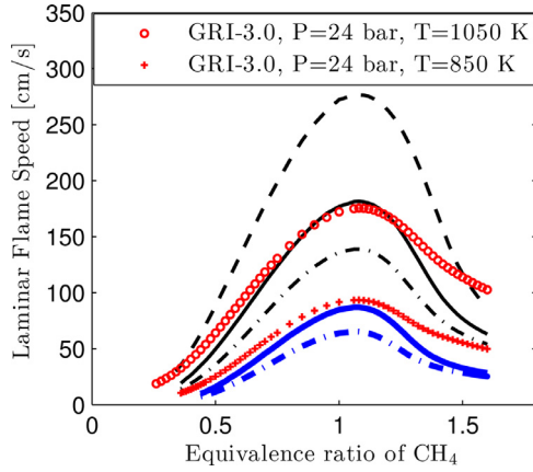
Fig. A.21. Laminar flame speeds computed using the Liu et al. (2004) skeletal scheme [20]. Curves as in Fig. 4.
